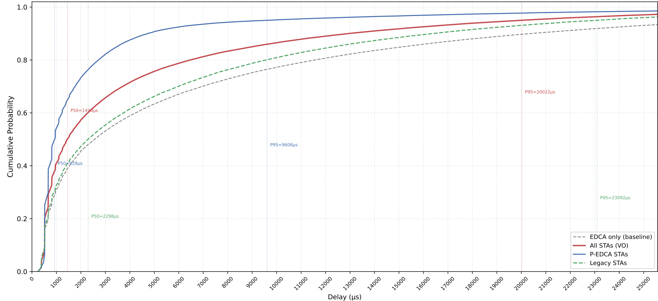
VO Delay CDF — P-EDCA / Legacy / All | CWds=1 × QSRC=0 × PSRC=3 nSta=30, nPedca=15/30, 1Mbps, avg of 10 runs
