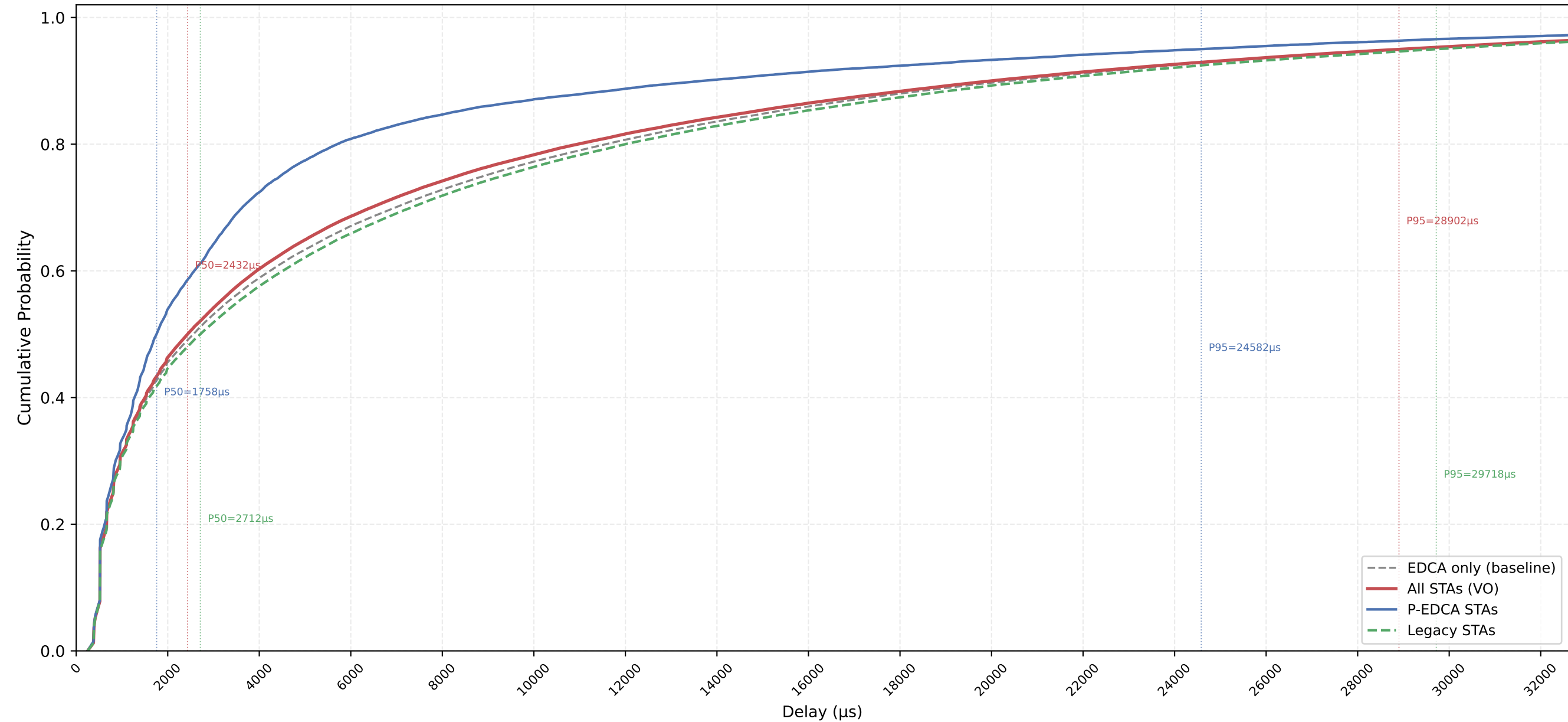
VO Delay CDF — P-EDCA / Legacy / All | CWds=1 × QSRC=1 × PSRC=1 nSta=30, nPedca=5/30, 1Mbps, avg of 10 runs
