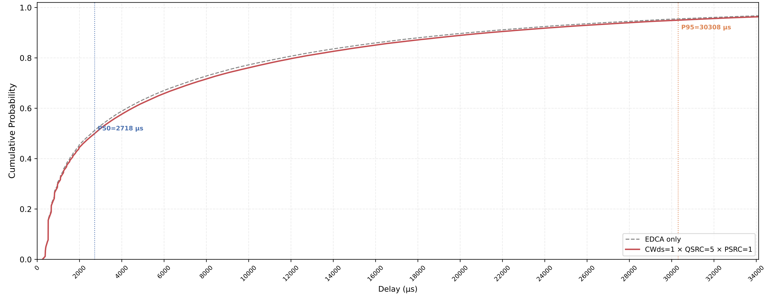
VO (all STAs) Delay CDF — CWds=1 × QSRC=5 × PSRC=1 nSta=30, nPedca=15, 1Mbps, avg of 10 runs
