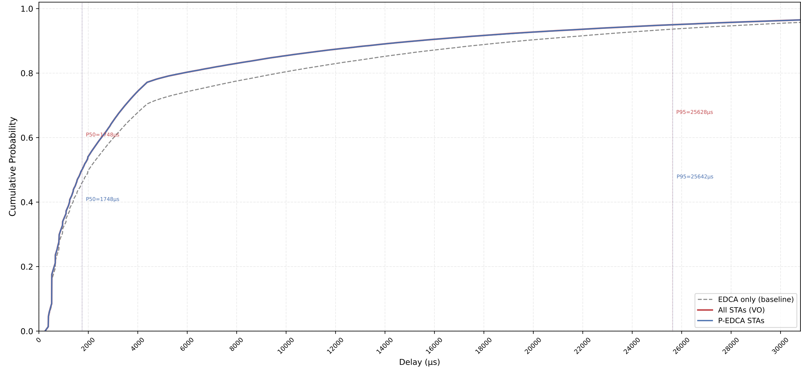
VO Delay CDF — P-EDCA / Legacy / All | CWds=0 × QSRC=2 × PSRC=1 nSta=30, nPedca=30/30, 1Mbps, avg of 10 runs
