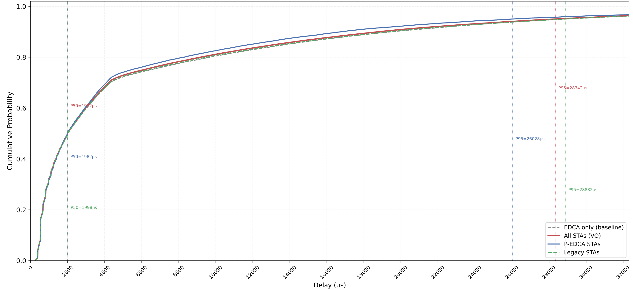
VO Delay CDF — P-EDCA / Legacy / All | CWds=0 × QSRC=4 × PSRC=2 nSta=30, nPedca=5/30, 1Mbps, avg of 10 runs
