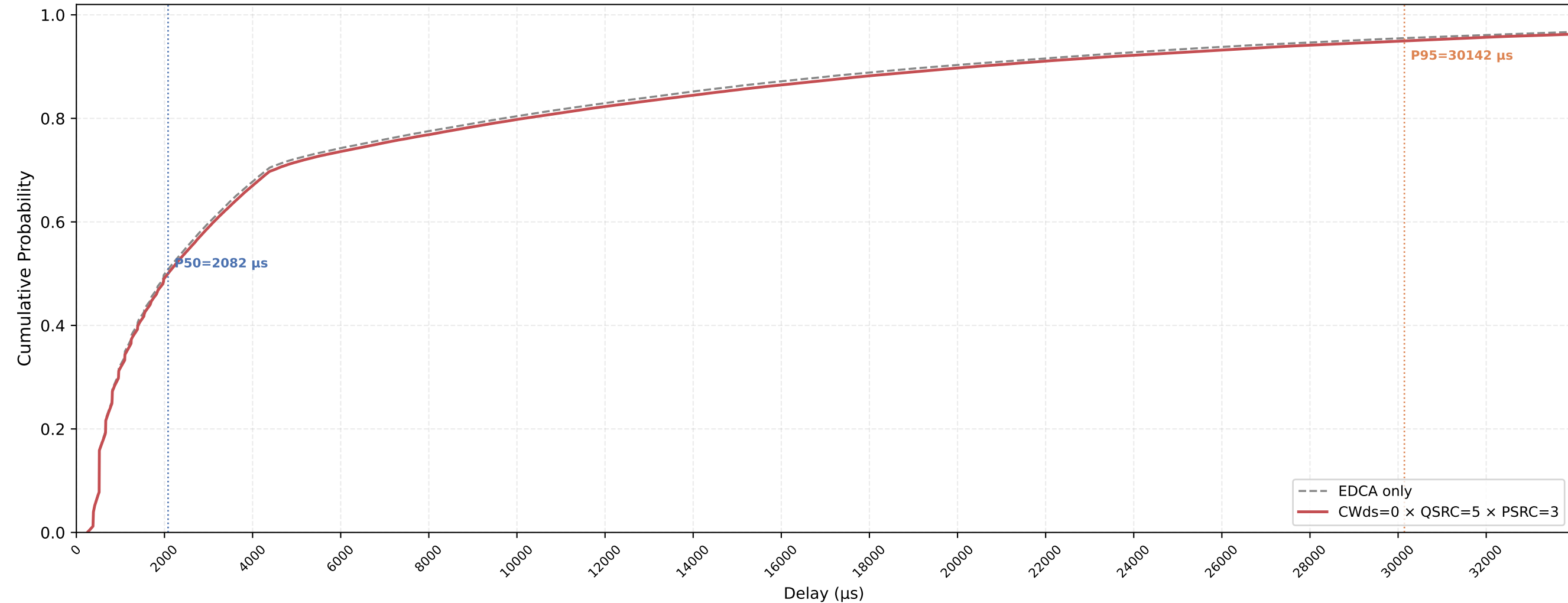
VO (all STAs) Delay CDF — CWds=0 × QSRC=5 × PSRC=3 nSta=30, nPedca=5, 1Mbps, avg of 10 runs
