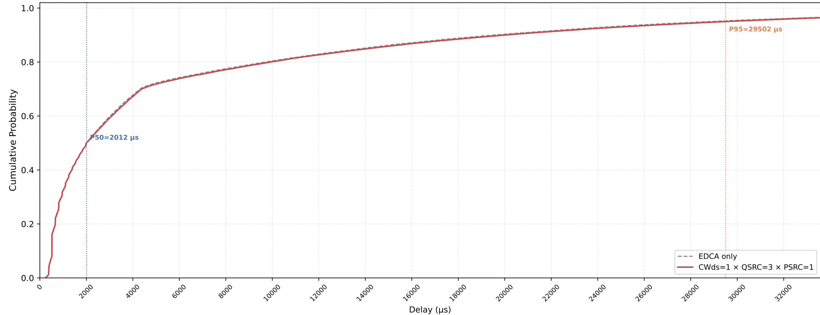
Legacy STA VO Delay CDF — CWds=1 × QSRC=3 × PSRC=1 nSta=30, nPedca=15, 1Mbps, avg of 10 runs
