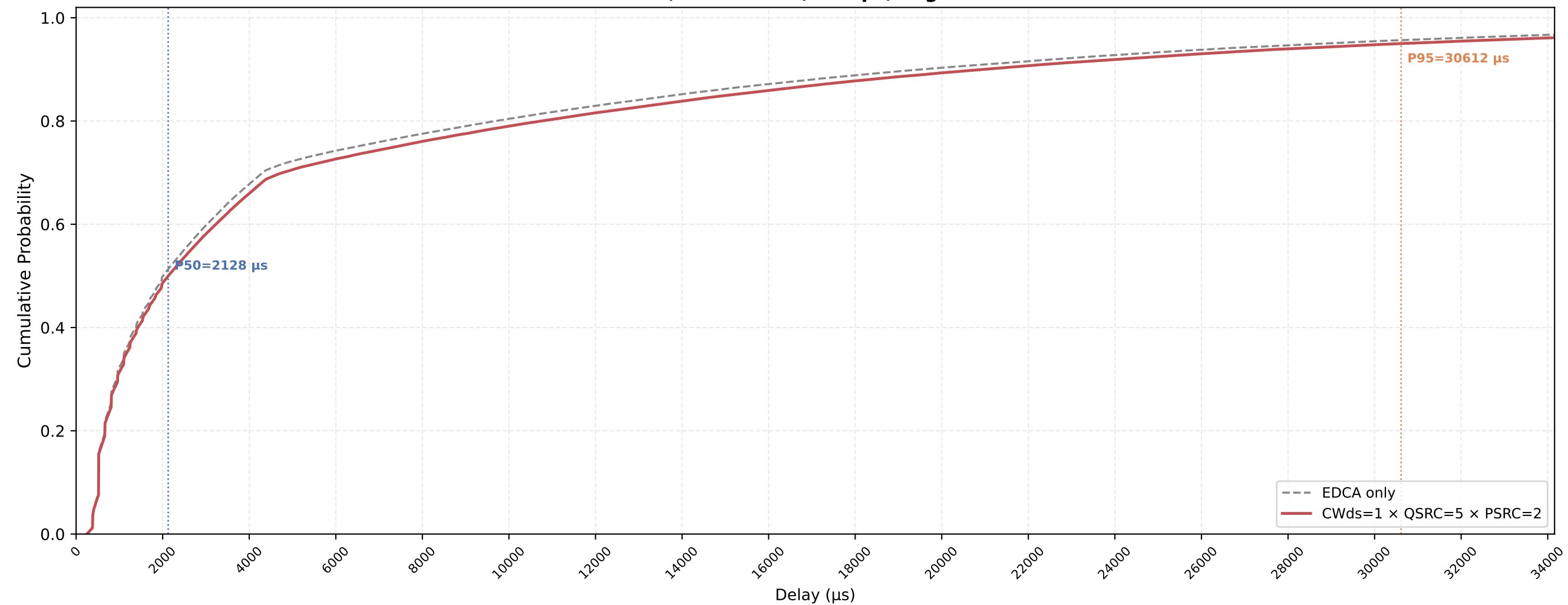
VO (all STAs) Delay CDF — CWds=1 × QSRC=5 × PSRC=2 nSta=30, nPedca=15, 1Mbps, avg of 10 runs
