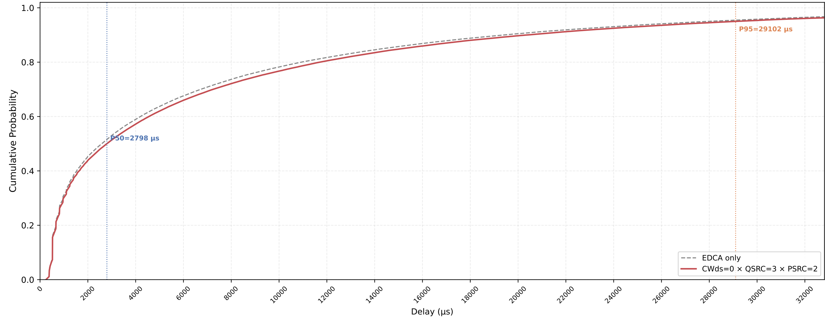
Legacy STA VO Delay CDF — CWds=0 × QSRC=3 × PSRC=2 nSta=30, nPedca=5, 1Mbps, avg of 10 runs
