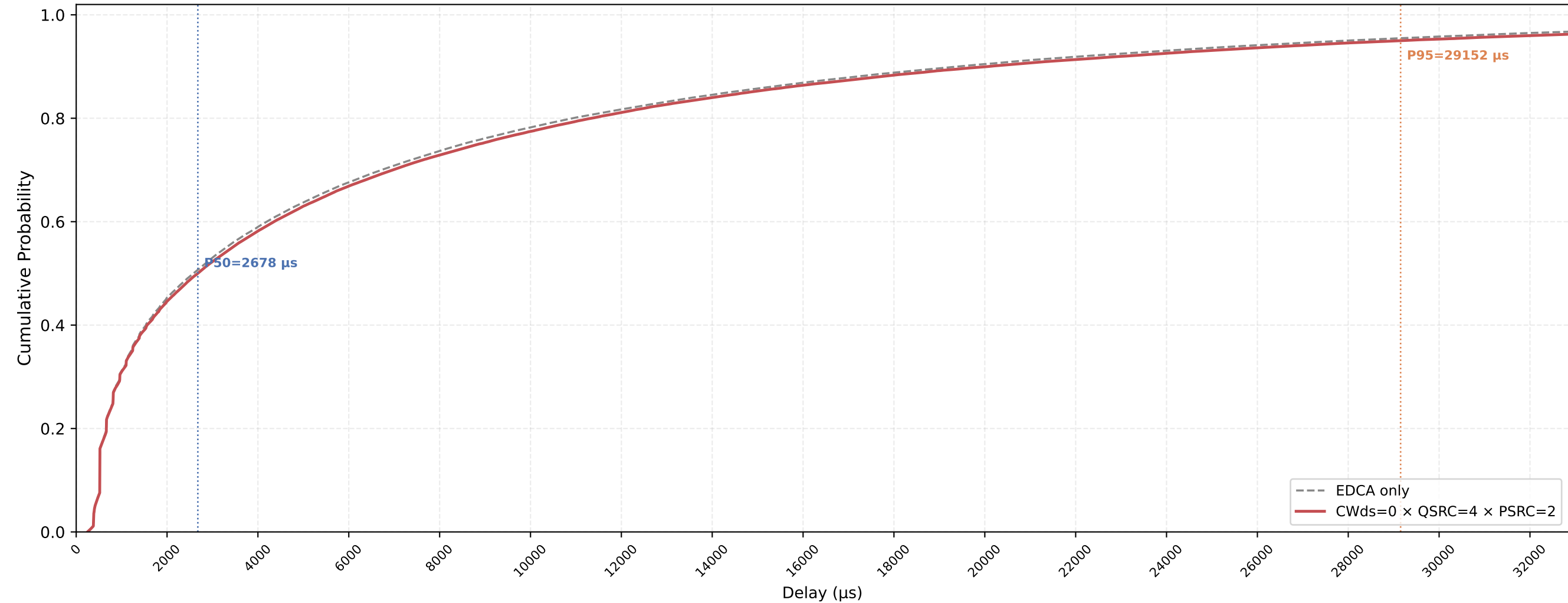
Legacy STA VO Delay CDF — CWds=0 × QSRC=4 × PSRC=2 nSta=30, nPedca=15, 1Mbps, avg of 10 runs
