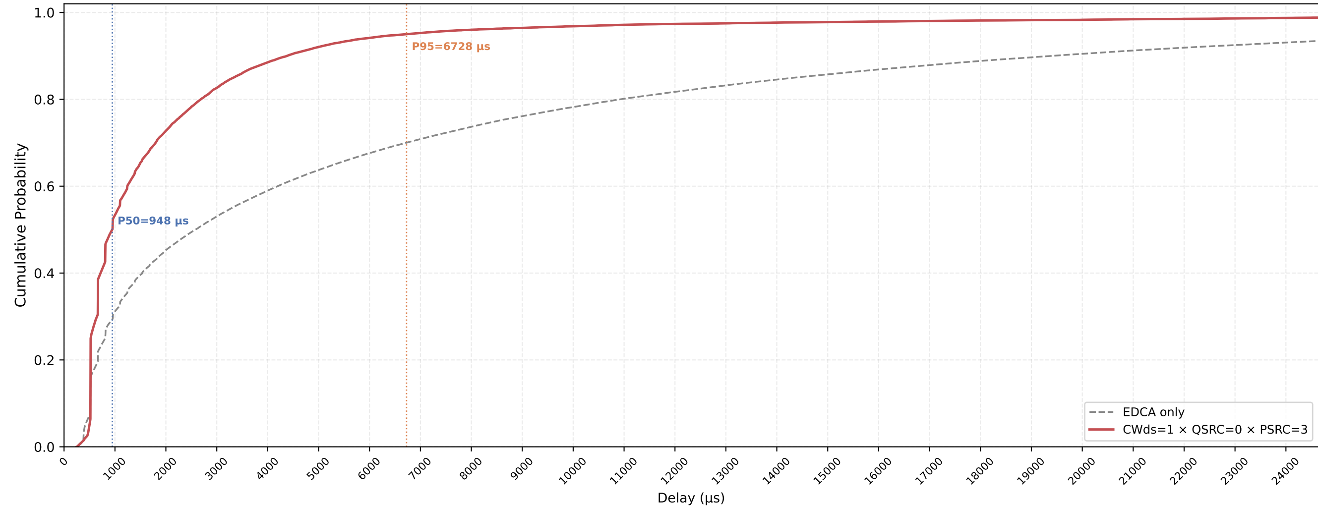
P-EDCA STA VO Delay CDF — CWds=1 × QSRC=0 × PSRC=3 nSta=30, nPedca=5, 1Mbps, avg of 10 runs
