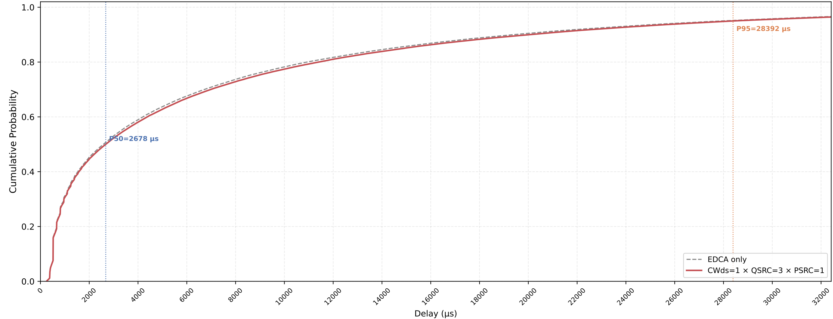
Legacy STA VO Delay CDF — CWds=1 × QSRC=3 × PSRC=1 nSta=30, nPedca=5, 1Mbps, avg of 10 runs
