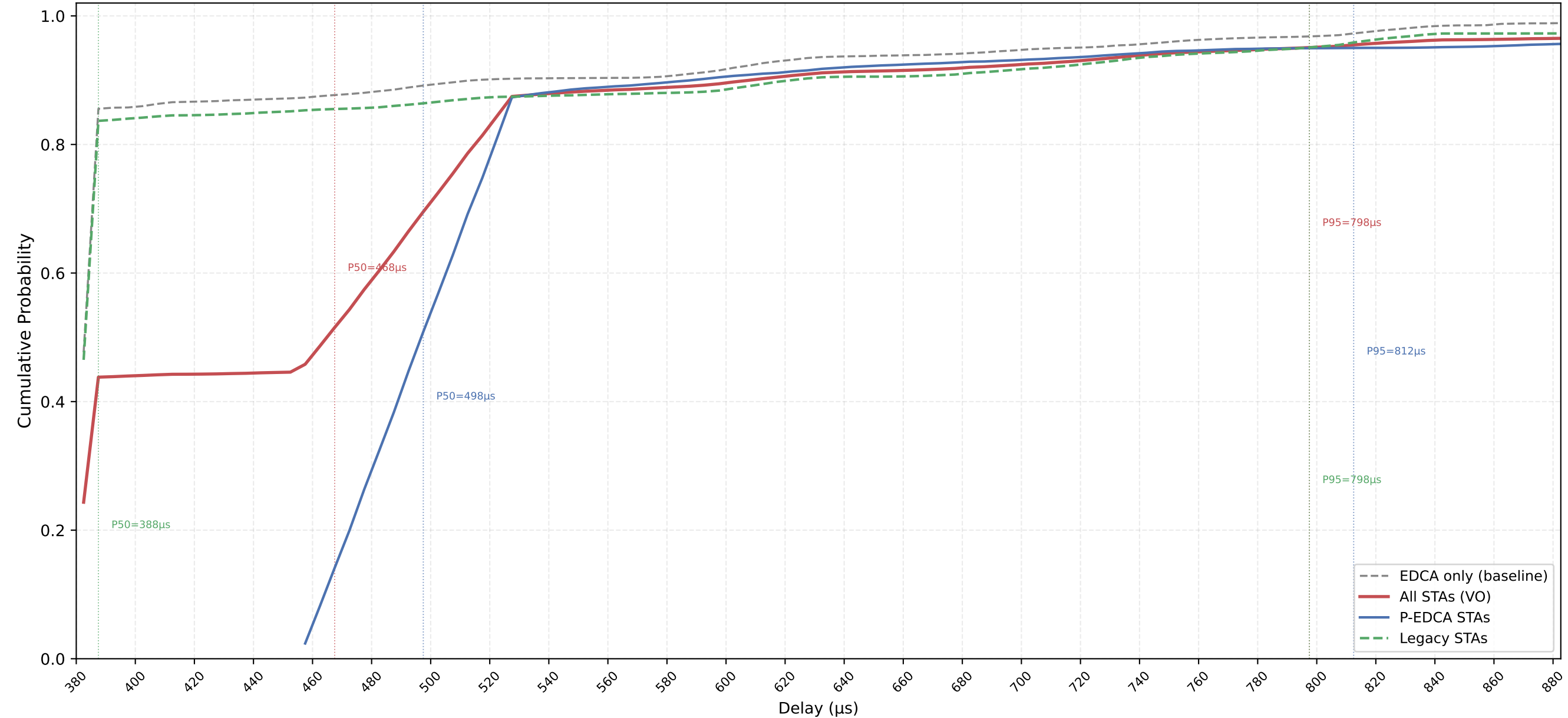
VO Delay CDF — P-EDCA / Legacy / All | CWds=0 × QSRC=0 × PSRC=1 nSta=30, nPedca=15/30, 0.1Mbps, avg of 10 runs
