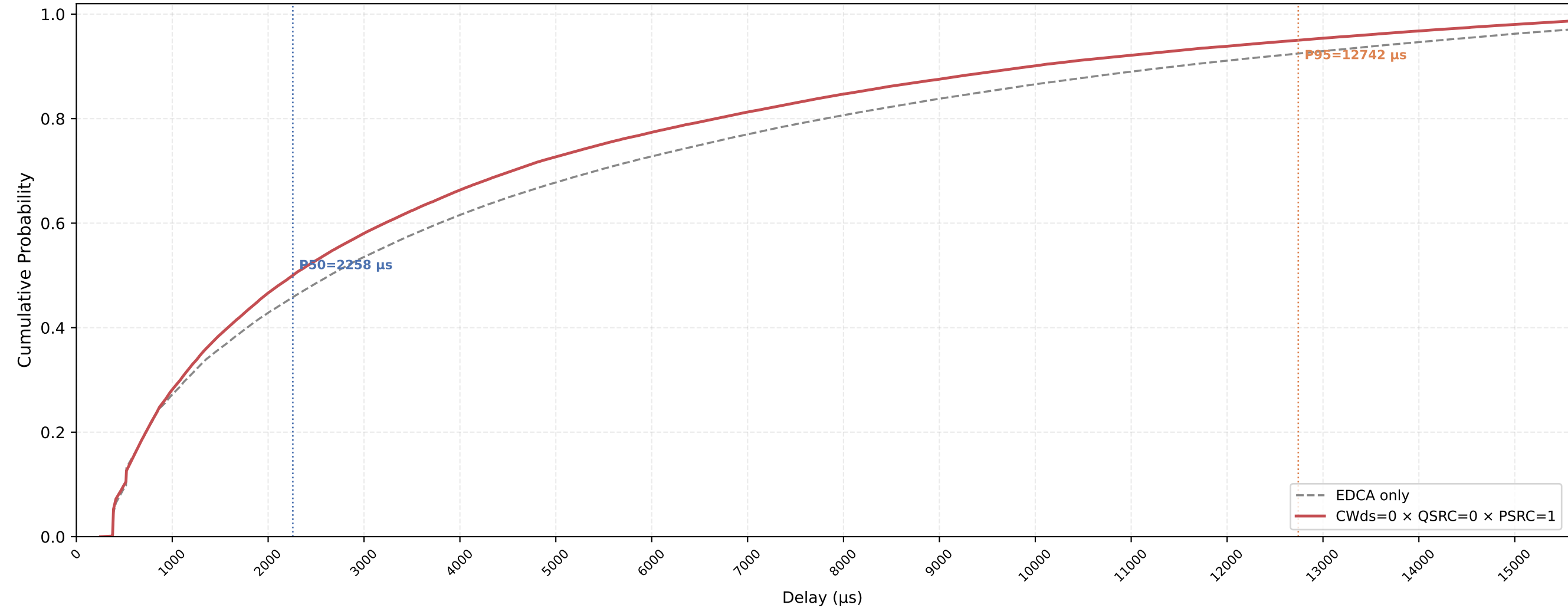
Legacy STA VO Delay CDF — CWds=0 × QSRC=0 × PSRC=1 nSta=30, nPedca=15, 0.5Mbps, avg of 10 runs
