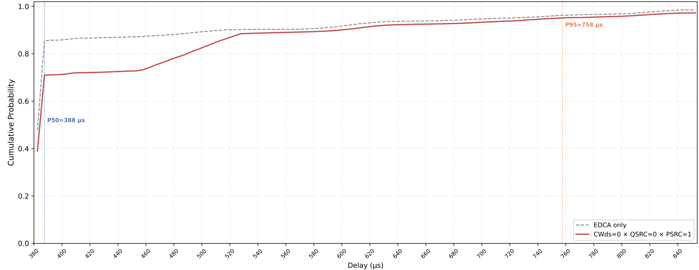
VO (all STAs) Delay CDF — CWds=0 × QSRC=0 × PSRC=1 nSta=30, nPedca=5, 0.1Mbps, avg of 10 runs
