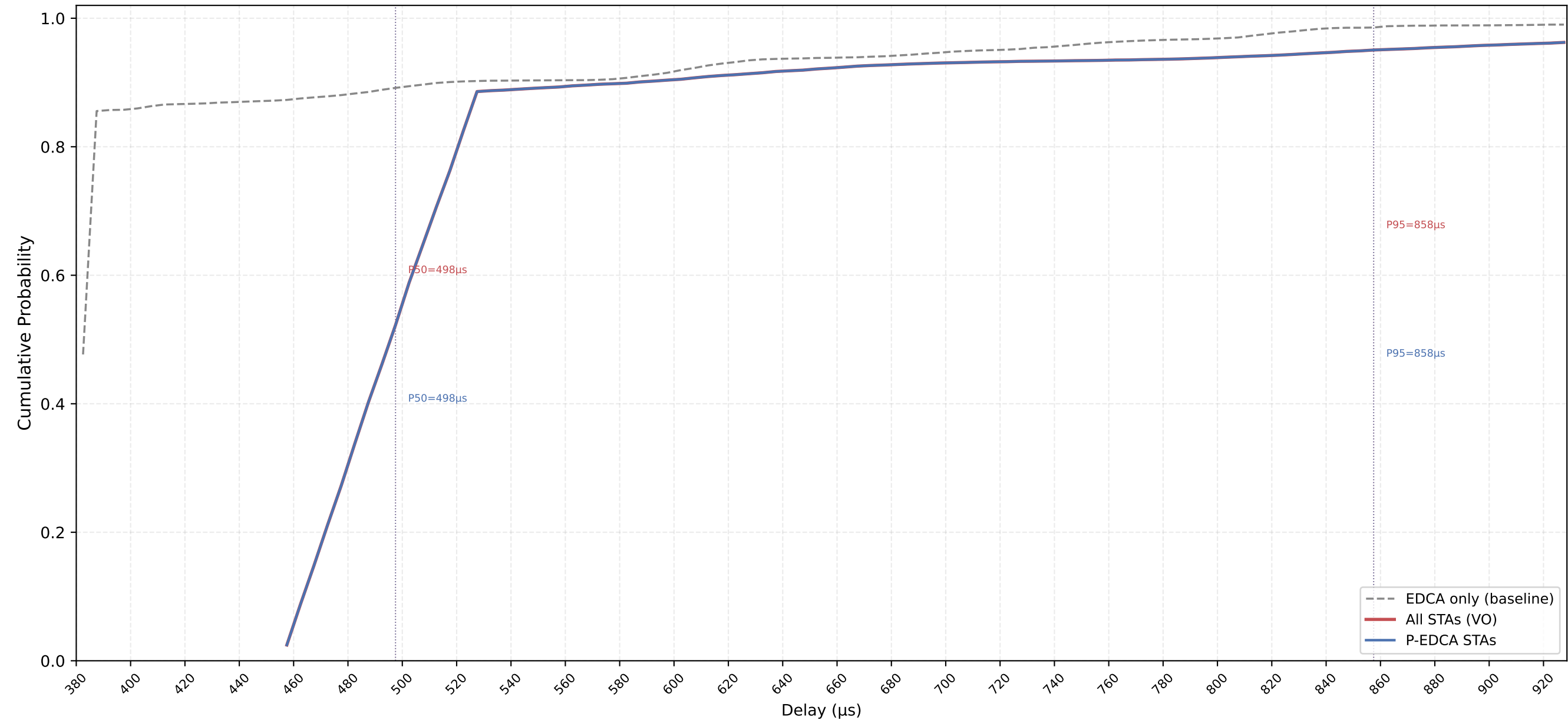
VO Delay CDF — P-EDCA / Legacy / All | CWds=0 × QSRC=0 × PSRC=3 nSta=30, nPedca=30/30, 0.1Mbps, avg of 10 runs
