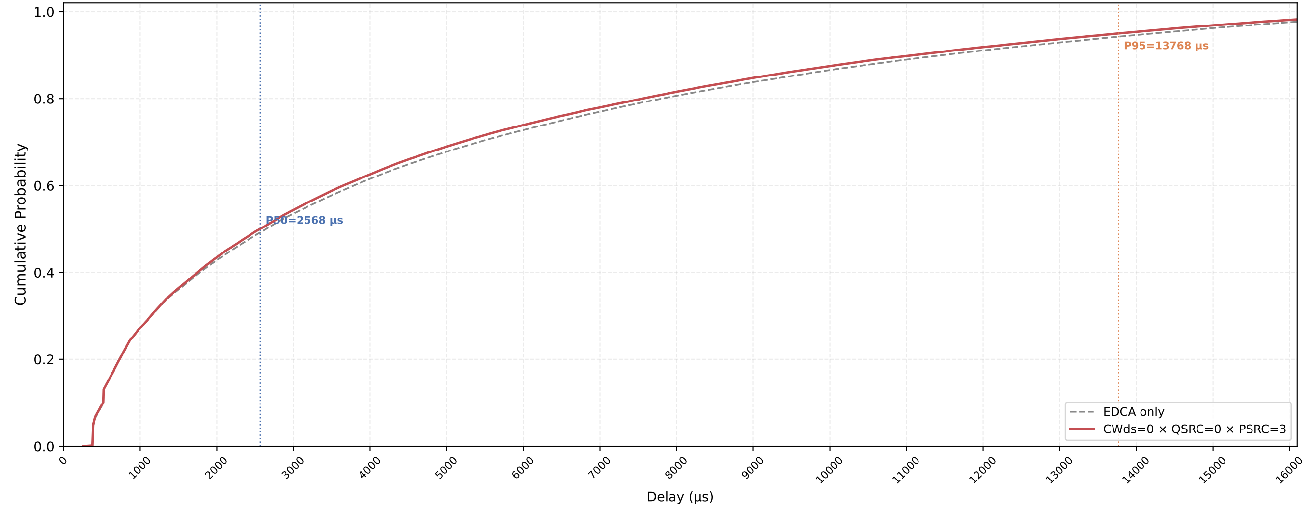
Legacy STA VO Delay CDF — CWds=0 × QSRC=0 × PSRC=3 nSta=30, nPedca=5, 0.5Mbps, avg of 10 runs
