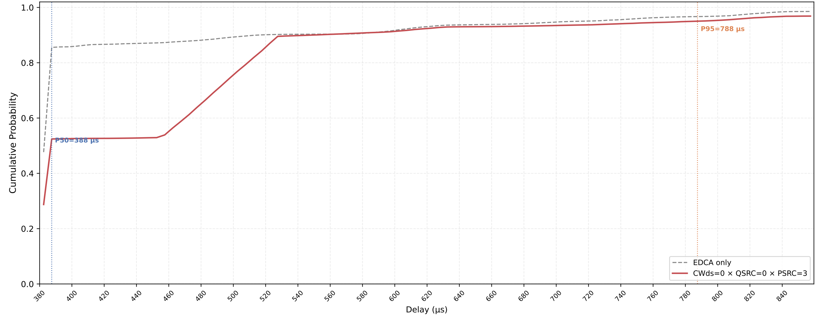
VO (all STAs) Delay CDF — CWds=0 × QSRC=0 × PSRC=3 nSta=30, nPedca=15, 0.1Mbps, avg of 10 runs
