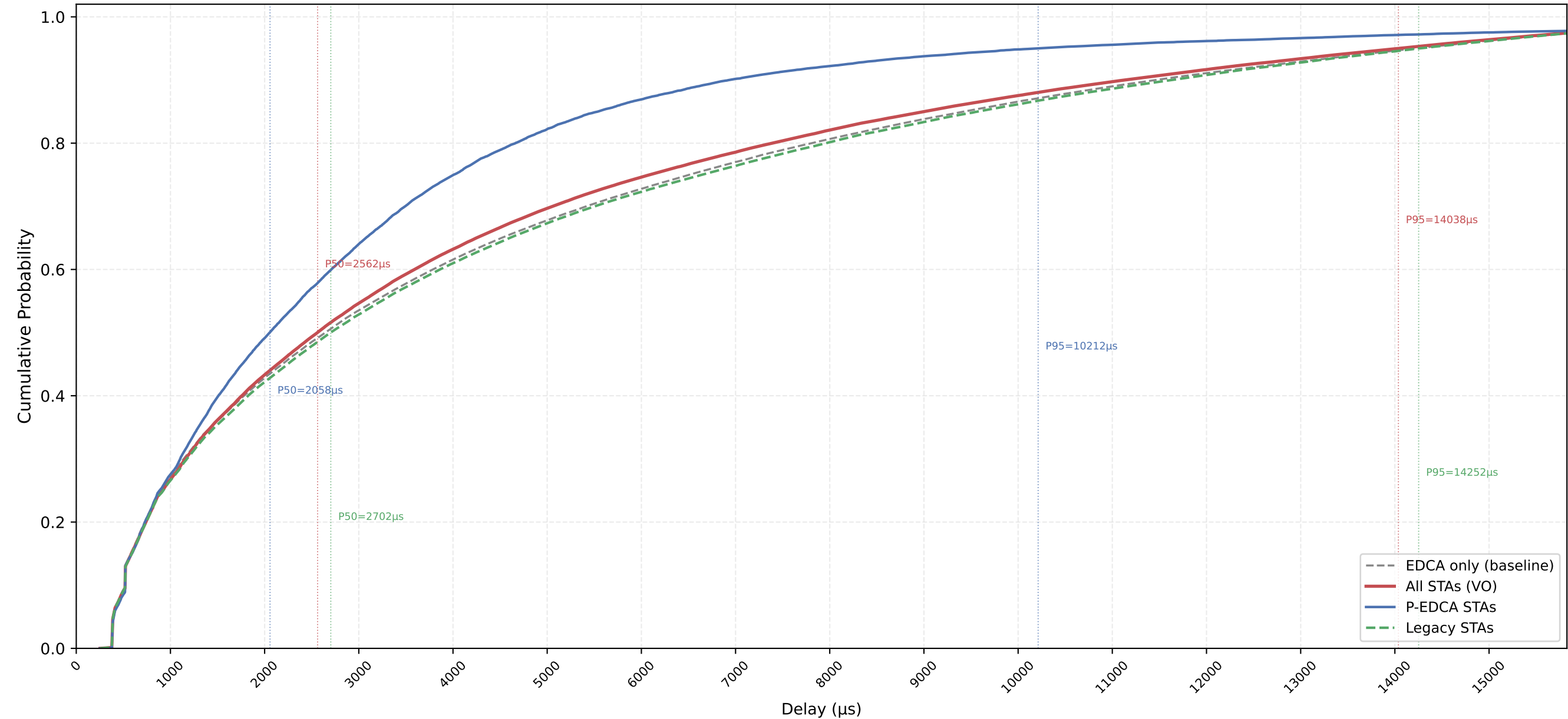
VO Delay CDF — P-EDCA / Legacy / All | CWds=0 × QSRC=1 × PSRC=1 nSta=30, nPedca=5/30, 0.5Mbps, avg of 10 runs
