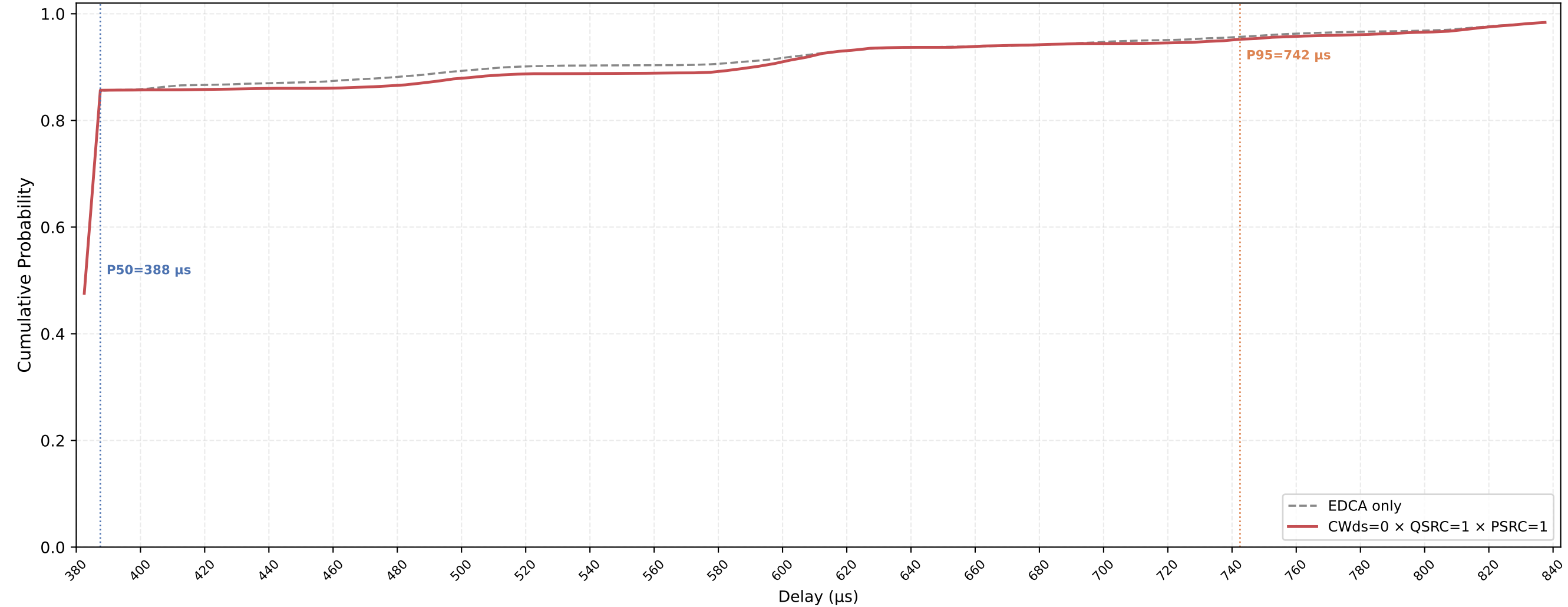
Legacy STA VO Delay CDF — CWds=0 × QSRC=1 × PSRC=1 nSta=30, nPedca=15, 0.1Mbps, avg of 10 runs
