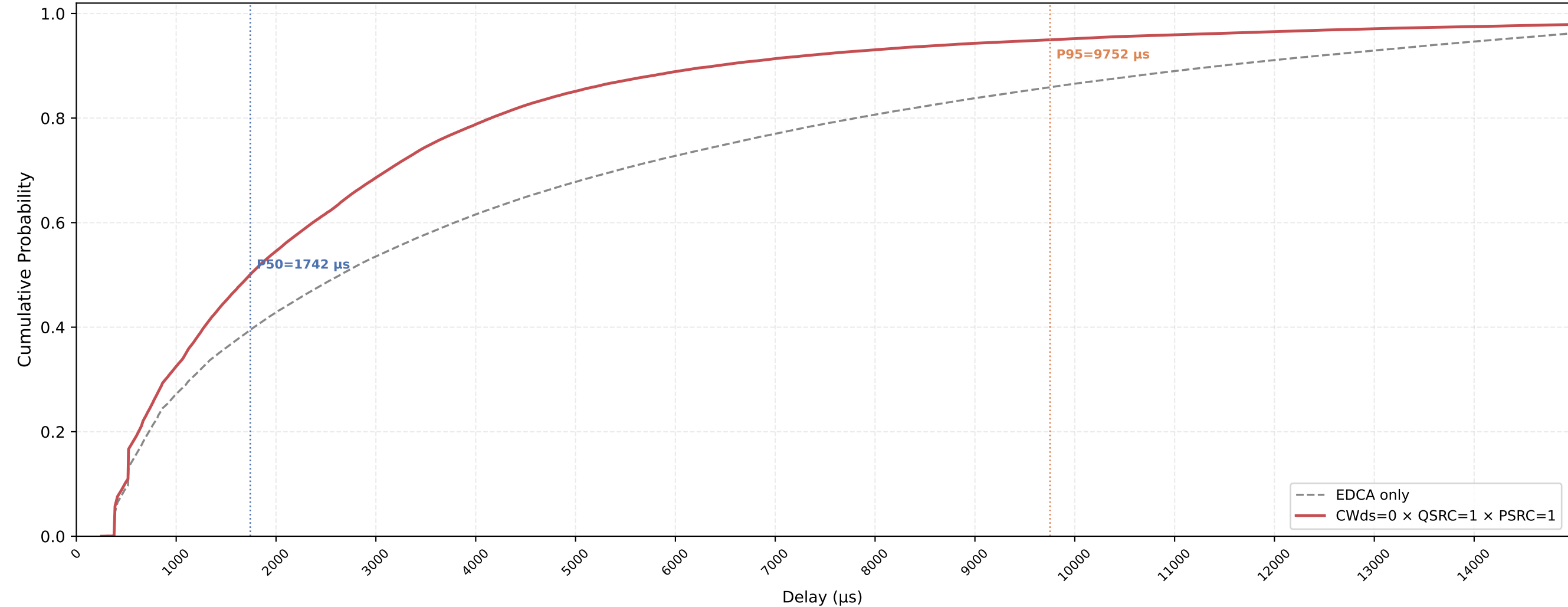
P-EDCA STA VO Delay CDF — CWds=0 × QSRC=1 × PSRC=1 nSta=30, nPedca=15, 0.5Mbps, avg of 10 runs
