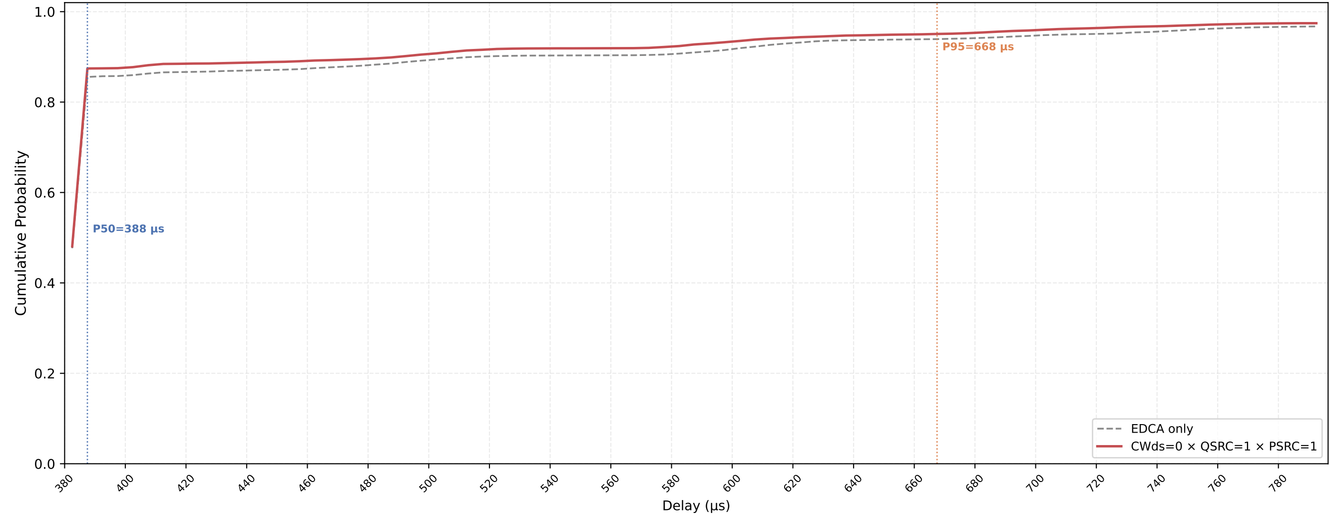
VO (all STAs) Delay CDF — CWds=0 × QSRC=1 × PSRC=1 nSta=30, nPedca=30, 0.1Mbps, avg of 10 runs
