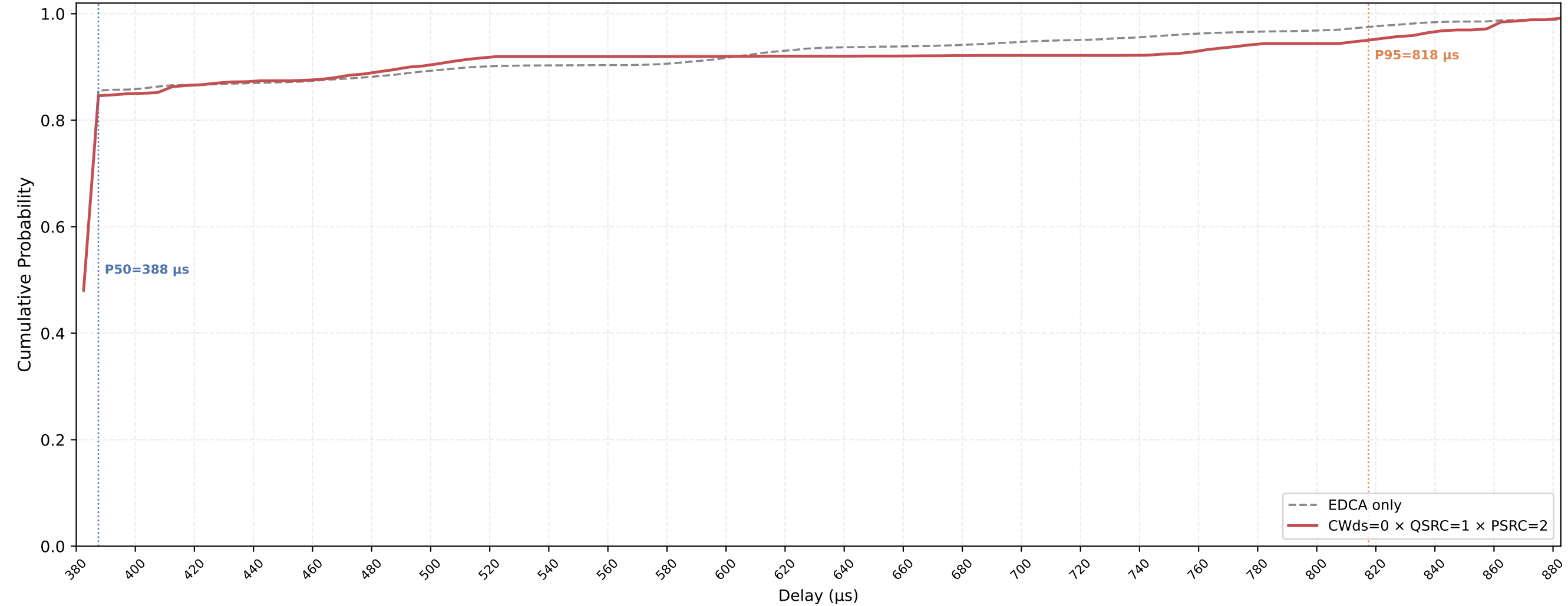
P-EDCA STA VO Delay CDF — CWds=0 × QSRC=1 × PSRC=2 nSta=30, nPedca=5, 0.1Mbps, avg of 10 runs
