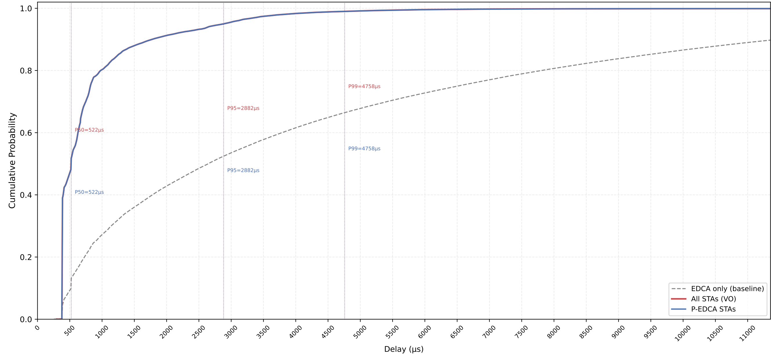
VO Delay CDF — P-EDCA / Legacy / All | CWds=0 × QSRC=1 × PSRC=3 nSta=30, nPedca=30/30, 0.5Mbps, avg of 10 runs
