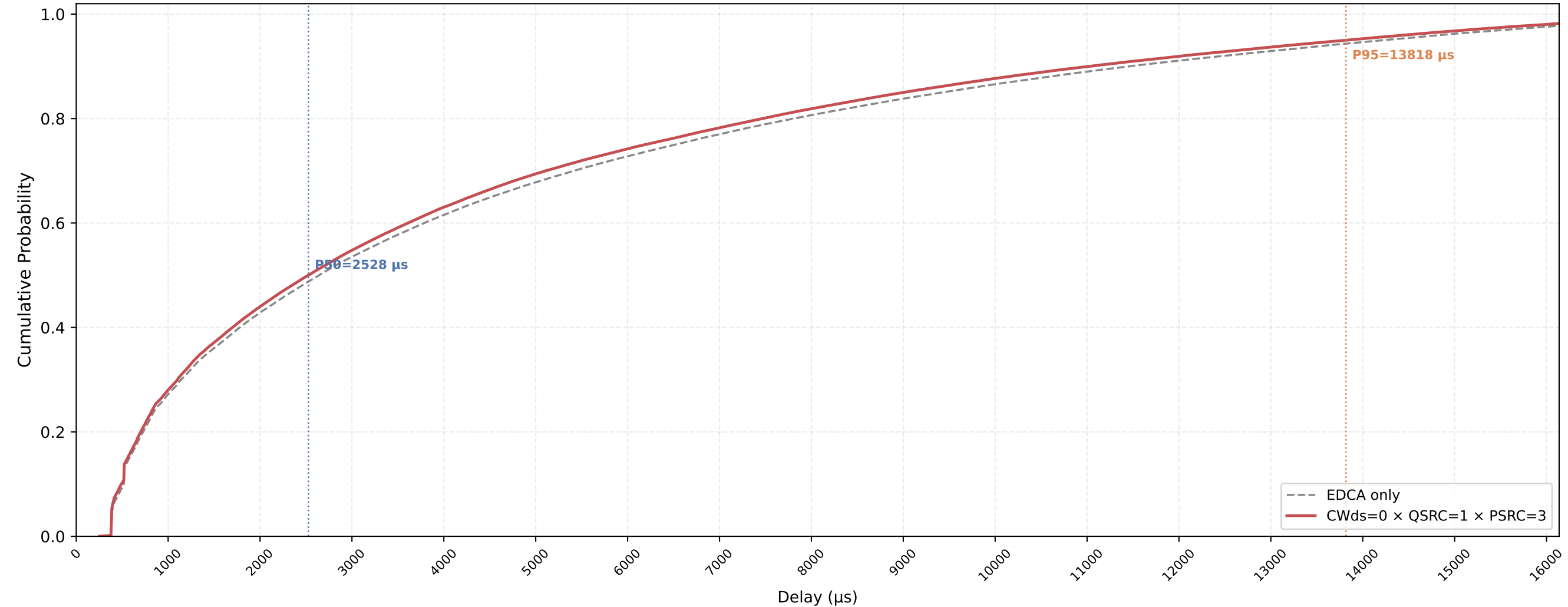
Legacy STA VO Delay CDF — CWds=0 × QSRC=1 × PSRC=3 nSta=30, nPedca=5, 0.5Mbps, avg of 10 runs
