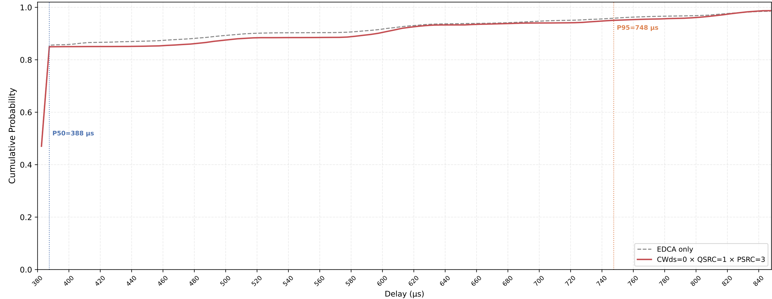
Legacy STA VO Delay CDF — CWds=0 × QSRC=1 × PSRC=3 nSta=30, nPedca=15, 0.1Mbps, avg of 10 runs
