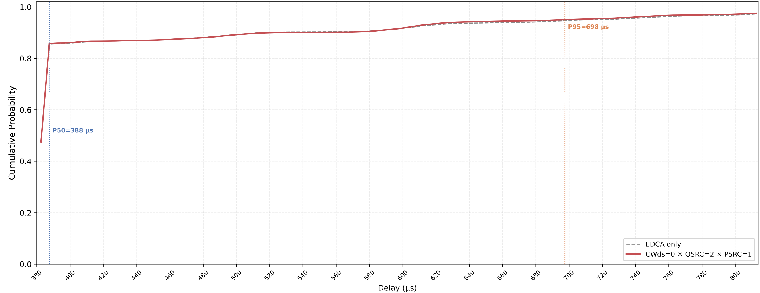
Legacy STA VO Delay CDF — CWds=0 × QSRC=2 × PSRC=1 nSta=30, nPedca=5, 0.1Mbps, avg of 10 runs
