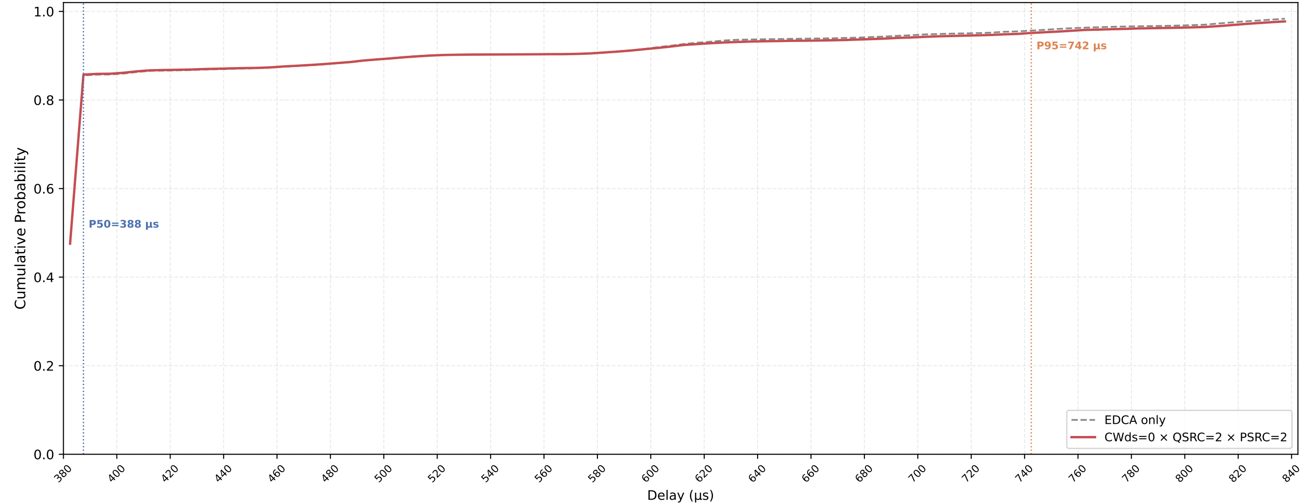
VO (all STAs) Delay CDF — CWds=0 × QSRC=2 × PSRC=2 nSta=30, nPedca=30, 0.1Mbps, avg of 10 runs
