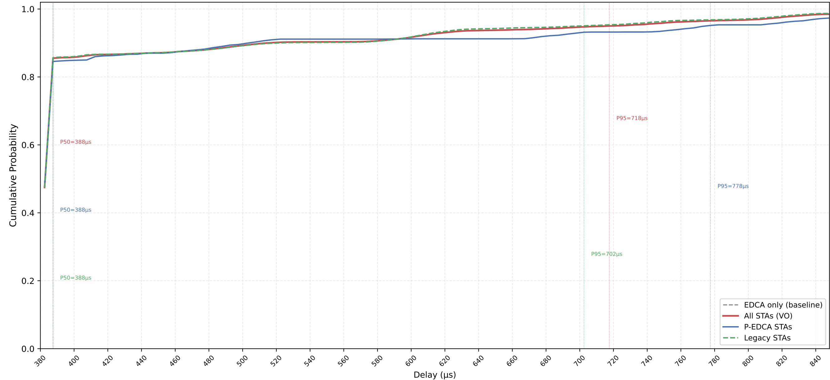
VO Delay CDF — P-EDCA / Legacy / All | CWds=0 × QSRC=2 × PSRC=3 nSta=30, nPedca=5/30, 0.1Mbps, avg of 10 runs
