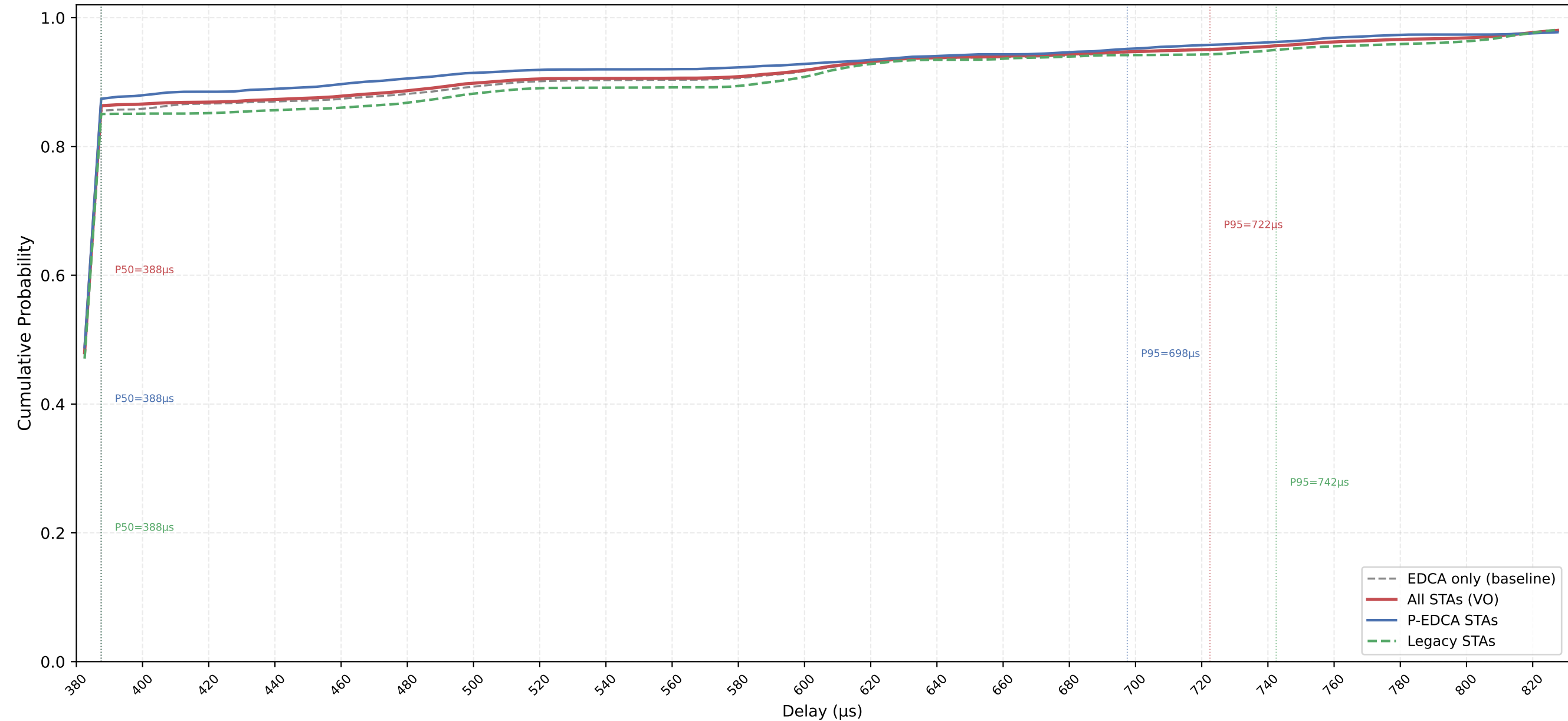
VO Delay CDF — P-EDCA / Legacy / All | CWds=0 × QSRC=2 × PSRC=3 nSta=30, nPedca=15/30, 0.1Mbps, avg of 10 runs
