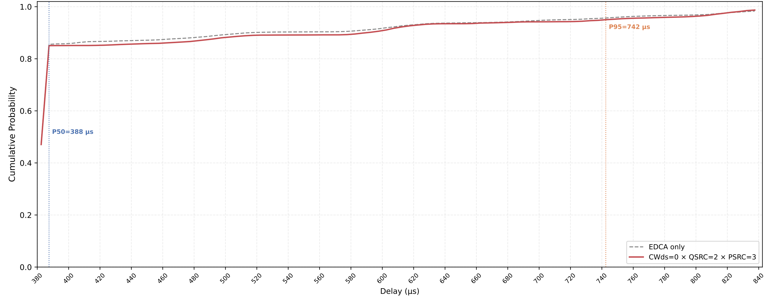
Legacy STA VO Delay CDF — CWds=0 × QSRC=2 × PSRC=3 nSta=30, nPedca=15, 0.1Mbps, avg of 10 runs
