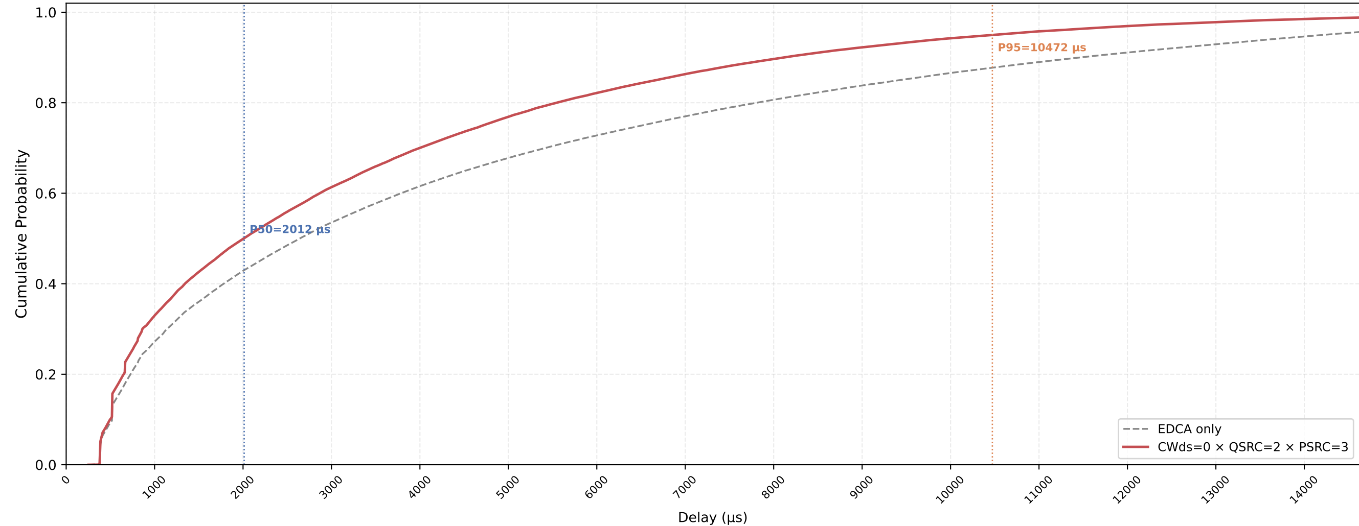
P-EDCA STA VO Delay CDF — CWds=0 × QSRC=2 × PSRC=3 nSta=30, nPedca=15, 0.5Mbps, avg of 10 runs
