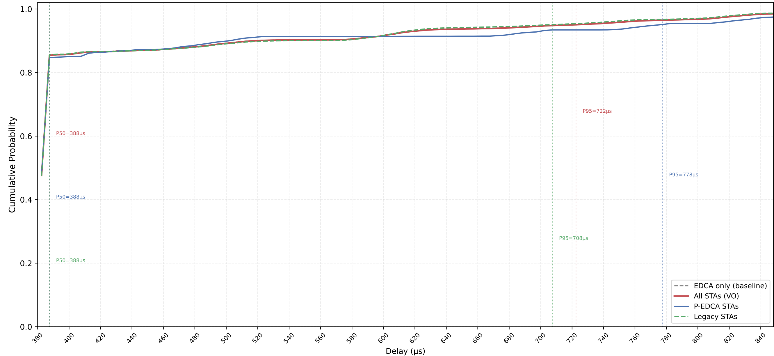
VO Delay CDF — P-EDCA / Legacy / All | CWds=0 × QSRC=3 × PSRC=1 nSta=30, nPedca=5/30, 0.1Mbps, avg of 10 runs
