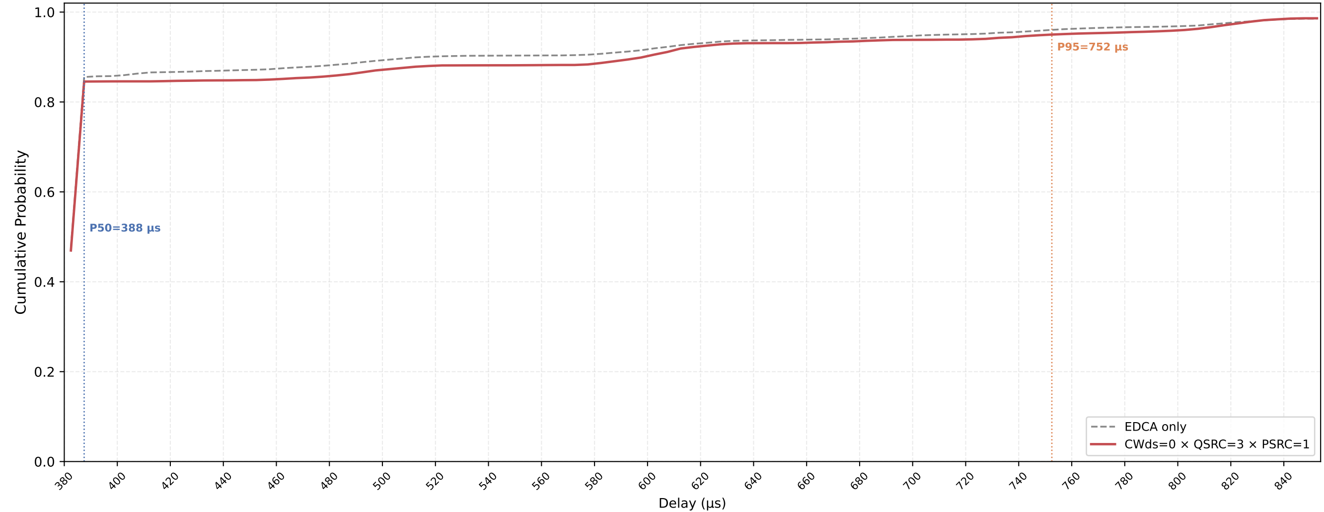
Legacy STA VO Delay CDF — CWds=0 × QSRC=3 × PSRC=1 nSta=30, nPedca=15, 0.1Mbps, avg of 10 runs
