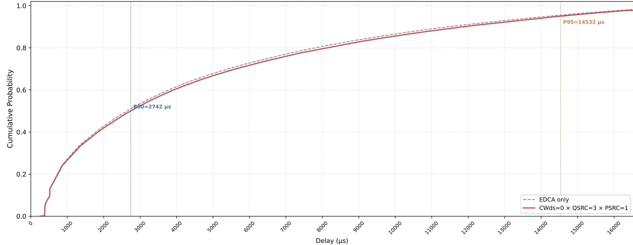
Legacy STA VO Delay CDF — CWds=0 × QSRC=3 × PSRC=1 nSta=30, nPedca=15, 0.5Mbps, avg of 10 runs
