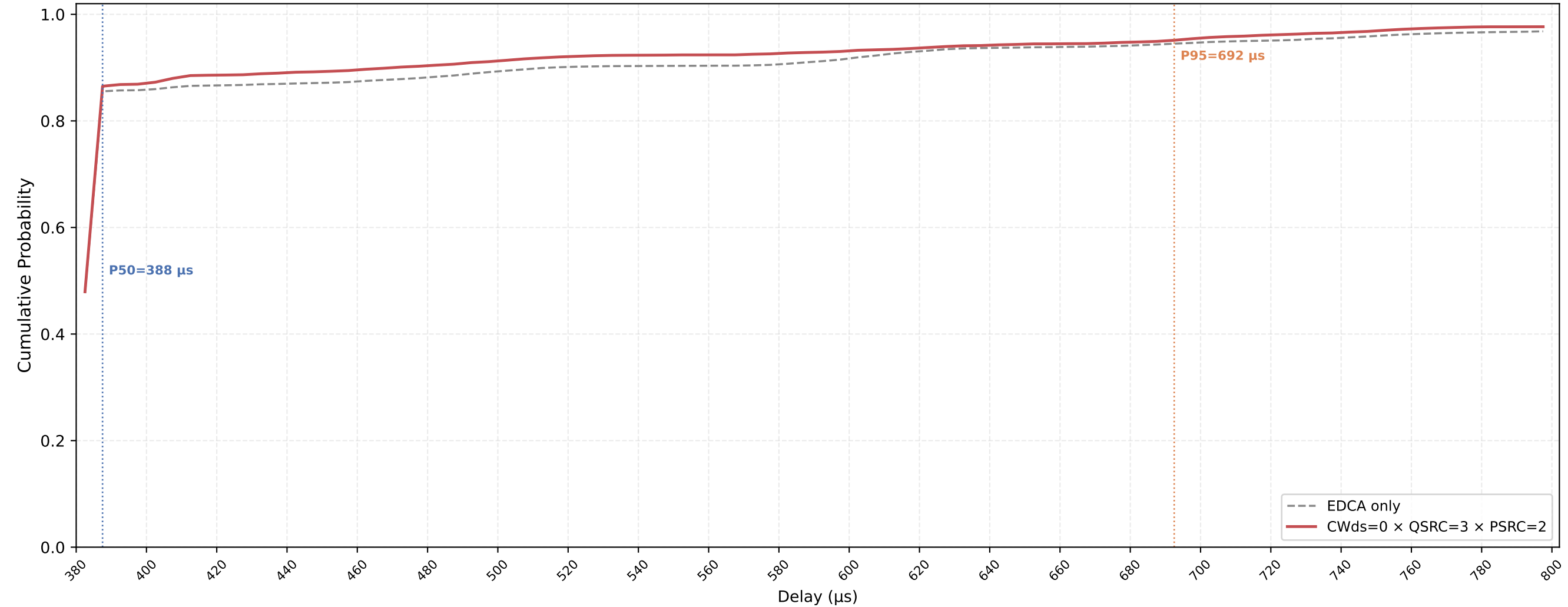
P-EDCA STA VO Delay CDF — CWds=0 × QSRC=3 × PSRC=2 nSta=30, nPedca=15, 0.1Mbps, avg of 10 runs
