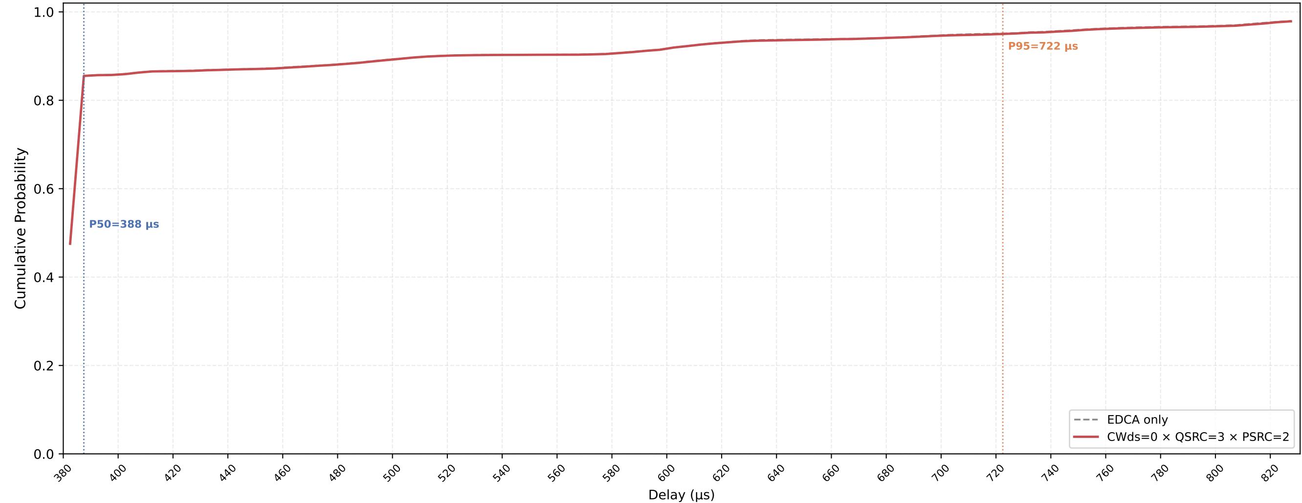
VO (all STAs) Delay CDF — CWds=0 × QSRC=3 × PSRC=2 nSta=30, nPedca=15, 0.1Mbps, avg of 10 runs
