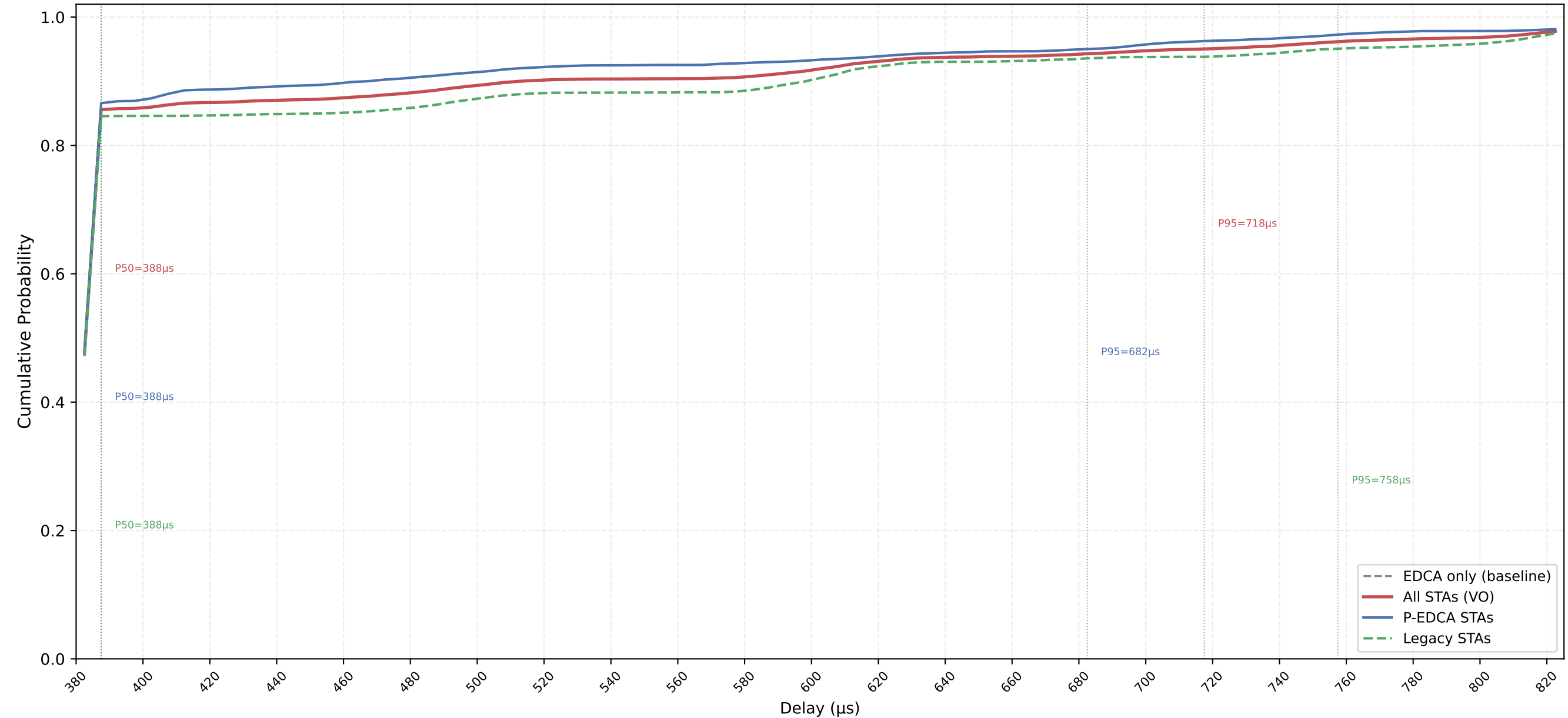
VO Delay CDF — P-EDCA / Legacy / All | CWds=0 × QSRC=4 × PSRC=1 nSta=30, nPedca=15/30, 0.1Mbps, avg of 10 runs
