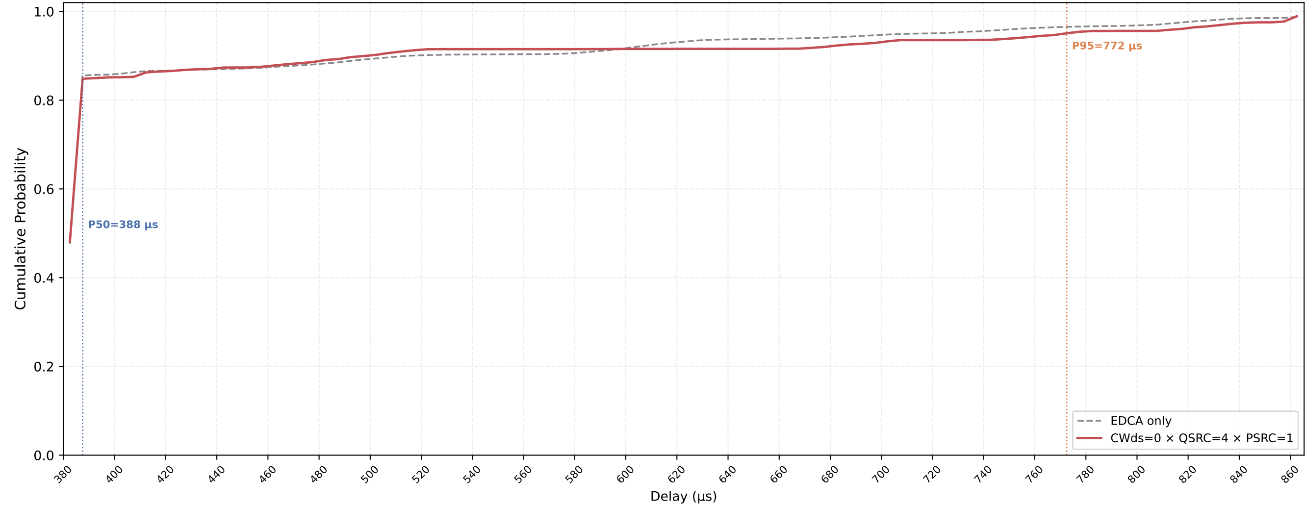
P-EDCA STA VO Delay CDF — CWds=0 × QSRC=4 × PSRC=1 nSta=30, nPedca=5, 0.1Mbps, avg of 10 runs
