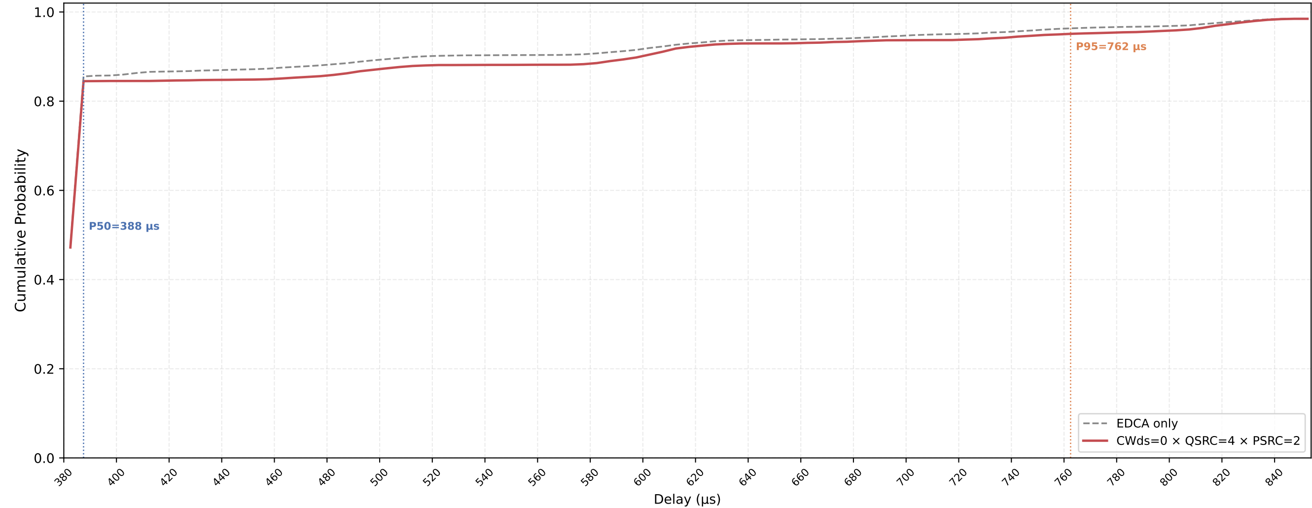
Legacy STA VO Delay CDF — CWds=0 × QSRC=4 × PSRC=2 nSta=30, nPedca=15, 0.1Mbps, avg of 10 runs
