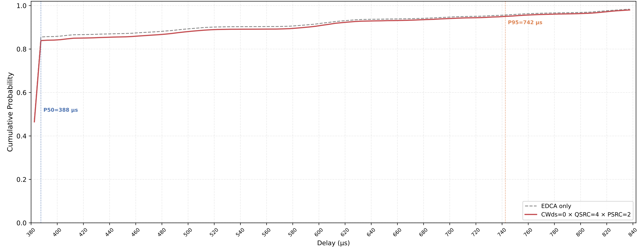
VO (all STAs) Delay CDF — CWds=0 × QSRC=4 × PSRC=2 nSta=30, nPedca=30, 0.1Mbps, avg of 10 runs
