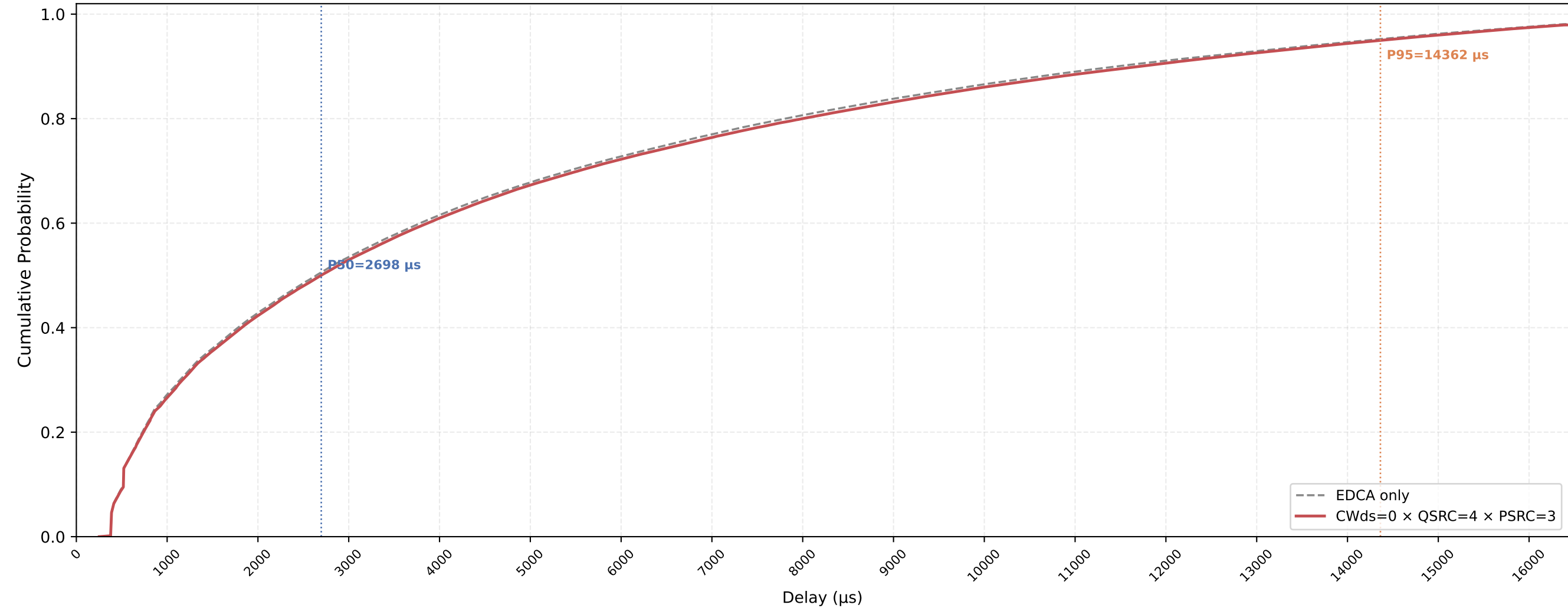
Legacy STA VO Delay CDF — CWds=0 × QSRC=4 × PSRC=3 nSta=30, nPedca=5, 0.5Mbps, avg of 10 runs
