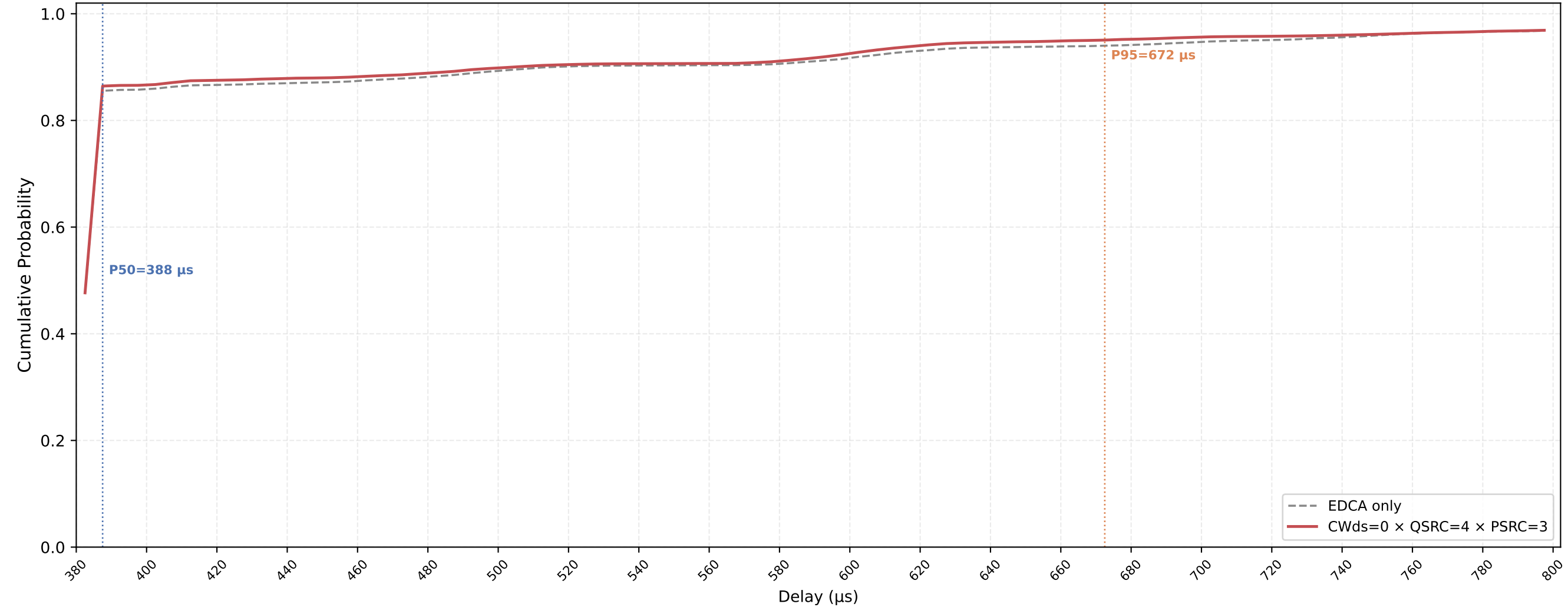
VO (all STAs) Delay CDF — CWds=0 × QSRC=4 × PSRC=3 nSta=30, nPedca=30, 0.1Mbps, avg of 10 runs
