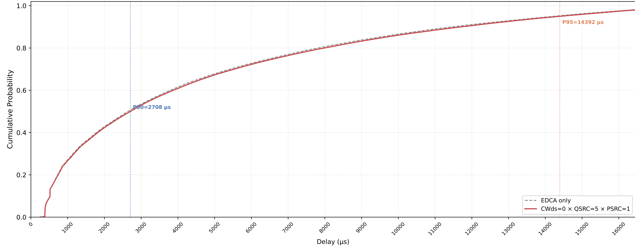
Legacy STA VO Delay CDF — CWds=0 × QSRC=5 × PSRC=1 nSta=30, nPedca=5, 0.5Mbps, avg of 10 runs
