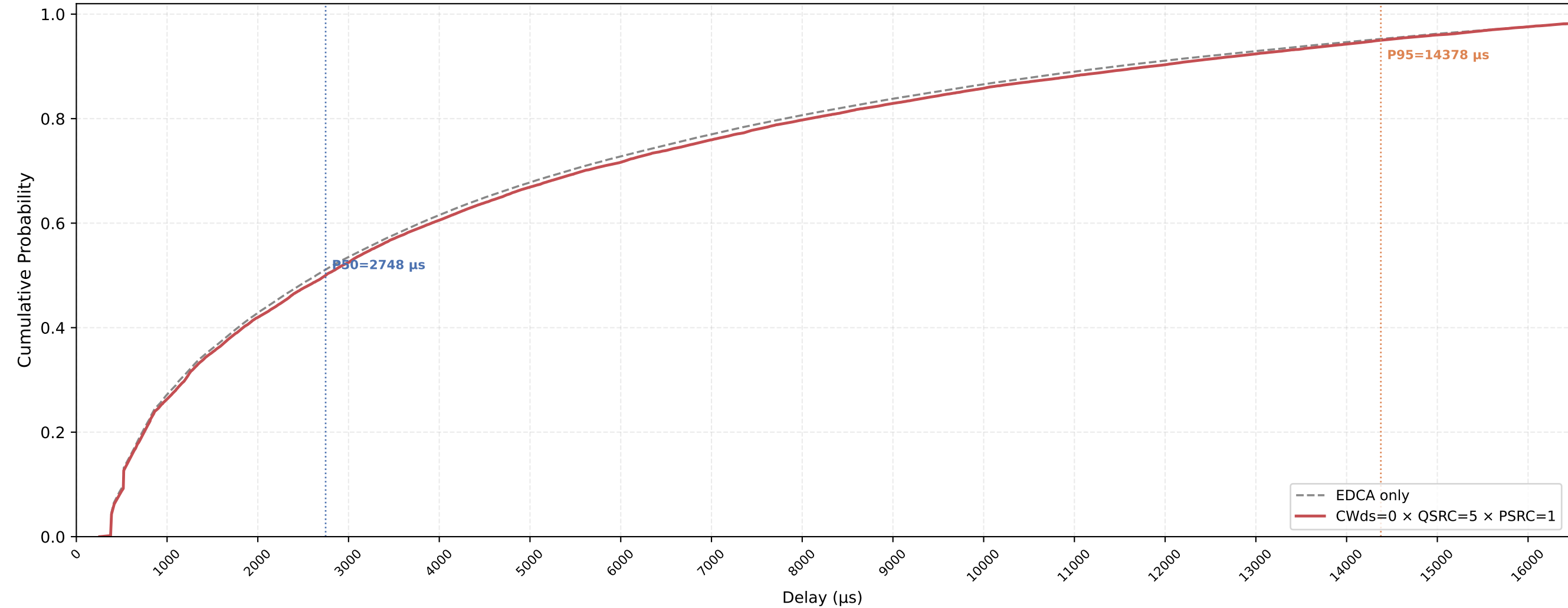
P-EDCA STA VO Delay CDF — CWds=0 × QSRC=5 × PSRC=1 nSta=30, nPedca=5, 0.5Mbps, avg of 10 runs
