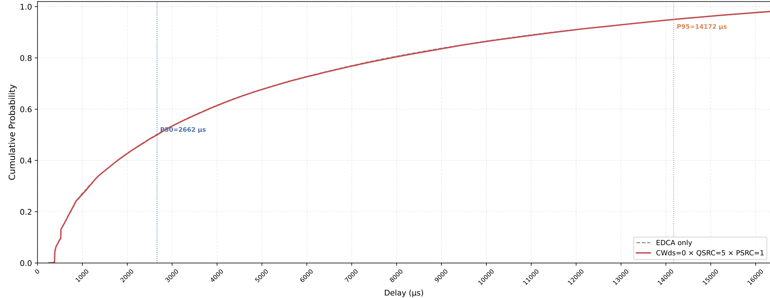
VO (all STAs) Delay CDF — CWds=0 × QSRC=5 × PSRC=1 nSta=30, nPedca=15, 0.5Mbps, avg of 10 runs
