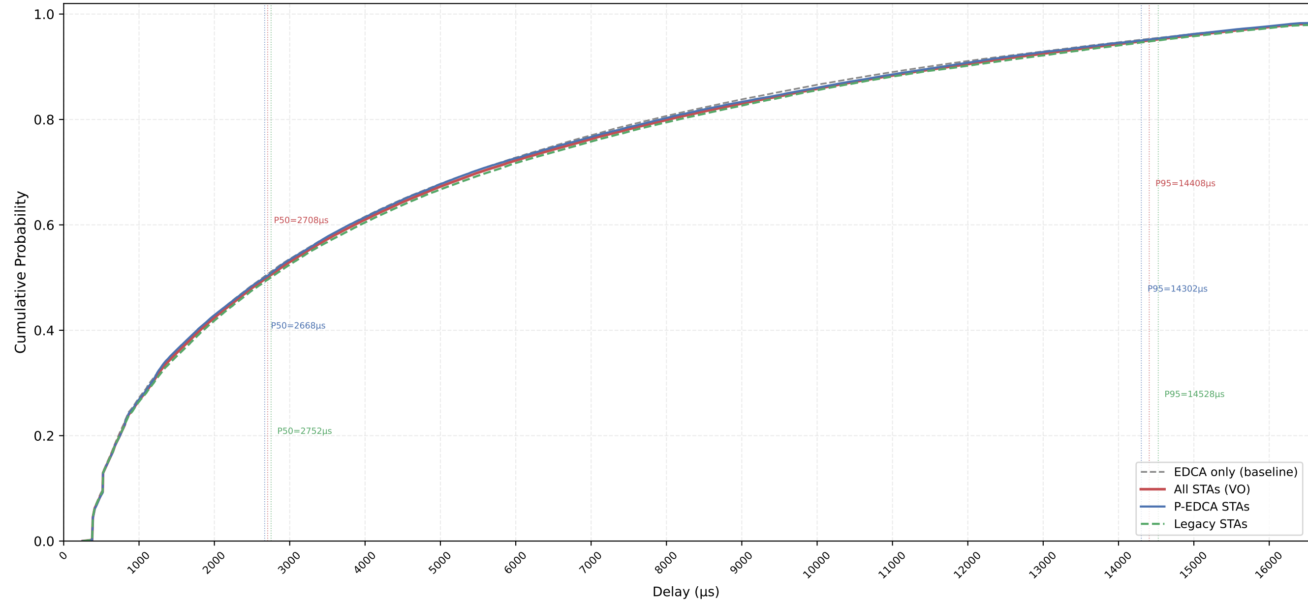
VO Delay CDF — P-EDCA / Legacy / All | CWds=0 × QSRC=5 × PSRC=2 nSta=30, nPedca=15/30, 0.5Mbps, avg of 10 runs
