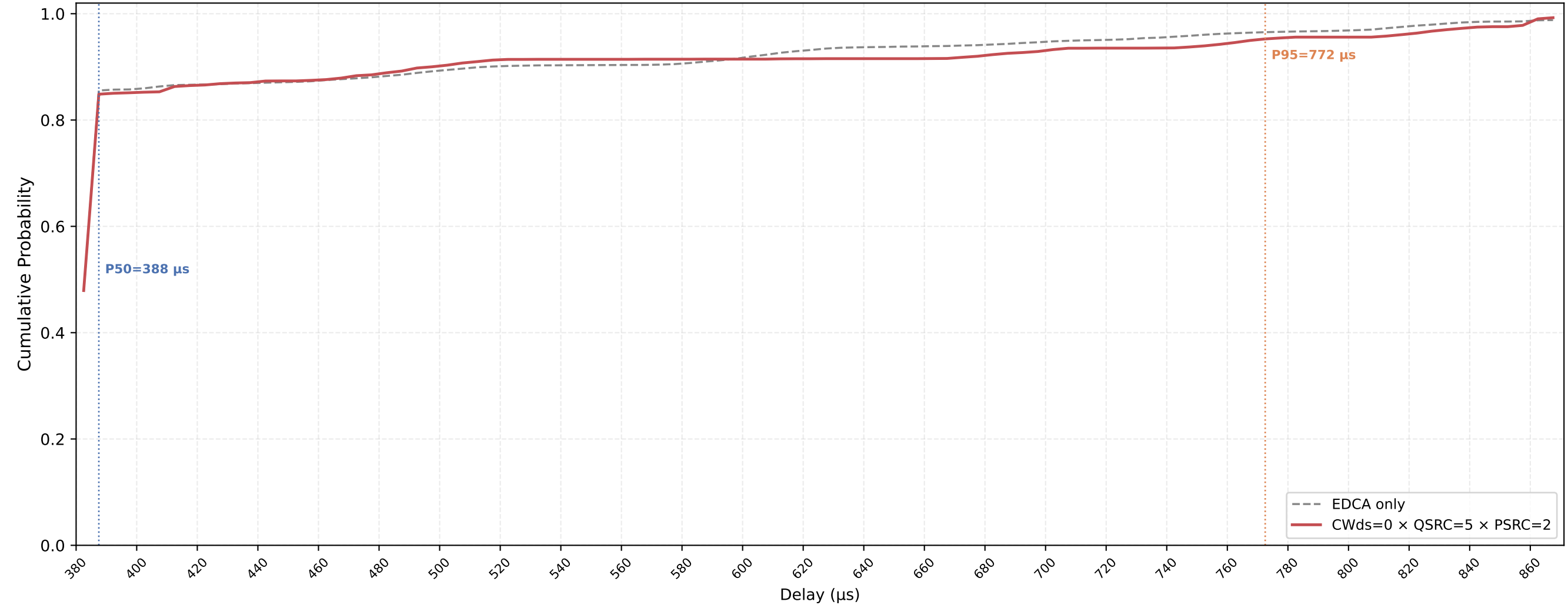
P-EDCA STA VO Delay CDF — CWds=0 × QSRC=5 × PSRC=2 nSta=30, nPedca=5, 0.1Mbps, avg of 10 runs
