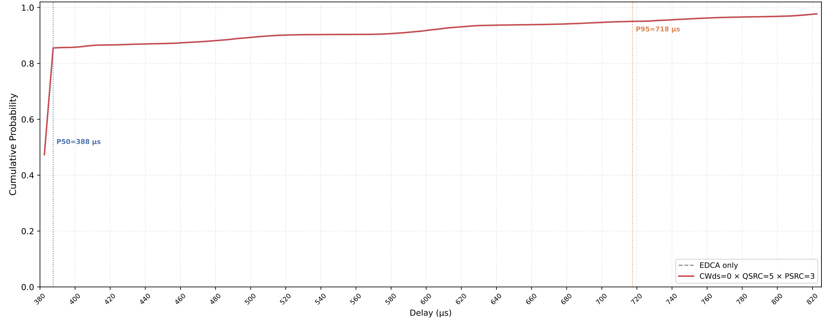
VO (all STAs) Delay CDF — CWds=0 × QSRC=5 × PSRC=3 nSta=30, nPedca=15, 0.1Mbps, avg of 10 runs
