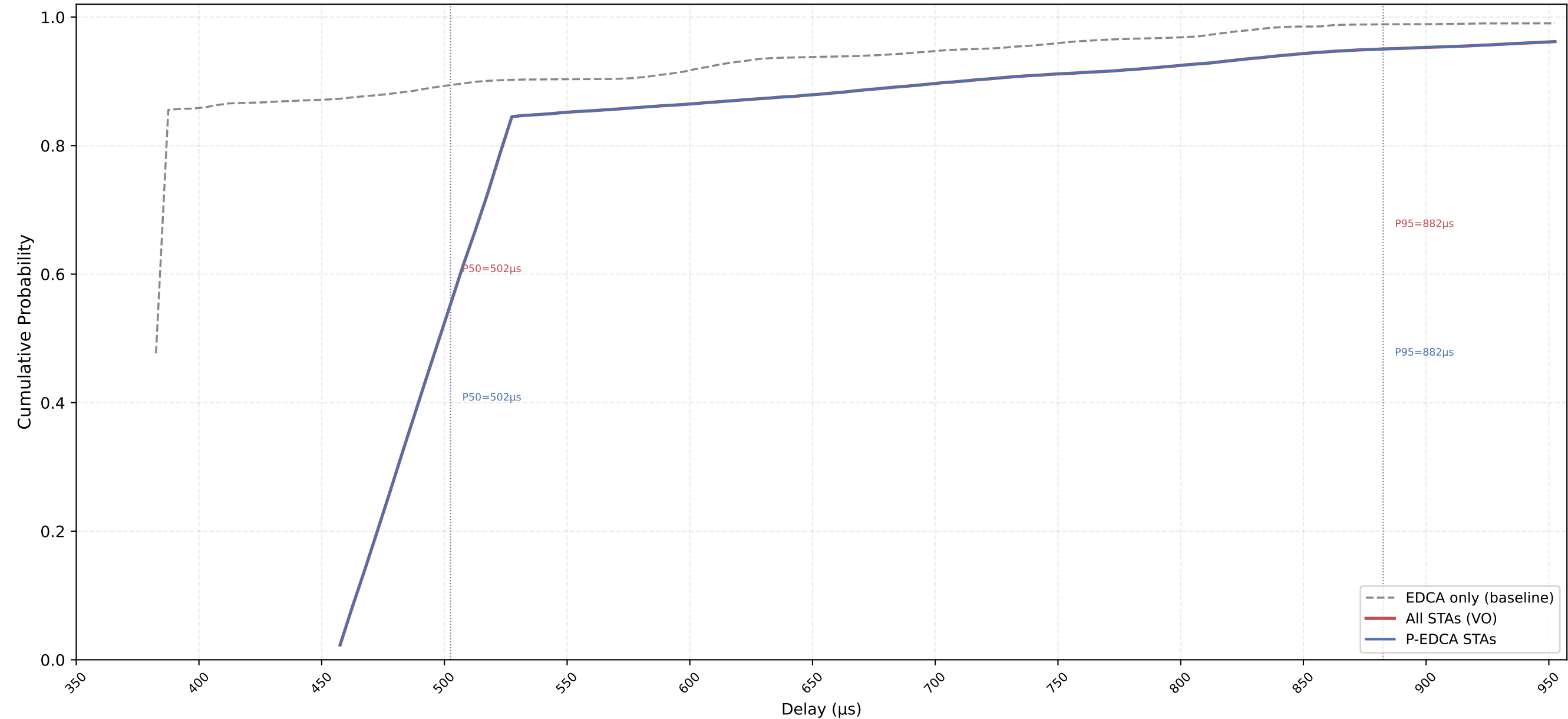
VO Delay CDF — P-EDCA / Legacy / All | CWds=1 × QSRC=0 × PSRC=1 nSta=30, nPedca=30/30, 0.1Mbps, avg of 10 runs
